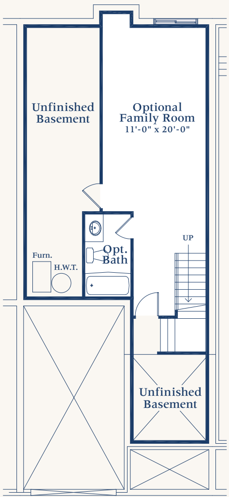
Optional Basement Floor Plan
