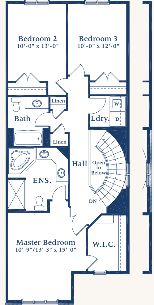
Second Floor Plan End Unit A (with brick)
